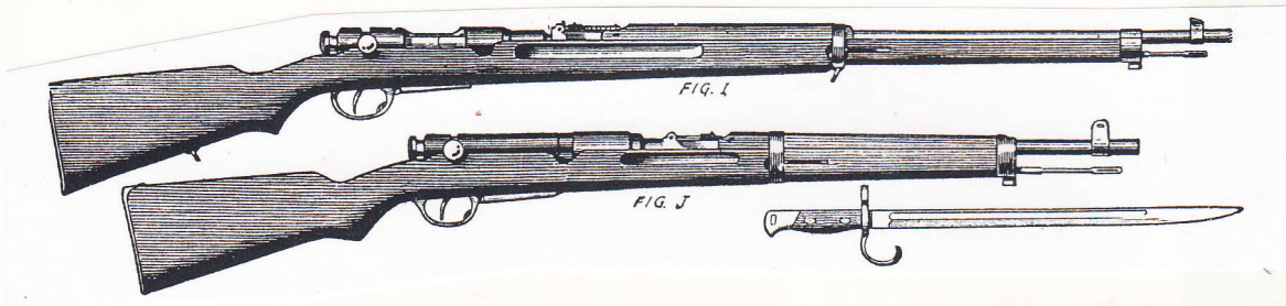
FIG. I. JAPAN ARISAKA MAGAZINE RIFLE. Model of 1907, officially known as "38th year model." Calibre is 6.5 m/m. or .256 inches. The magazine is a copy of the Mauser with a few changes. A dust-cover easily attached is part of the equipment. The bayonet resembles the English bayonet of 1903. Thousands of these rifles were sold by Japan to Russia during the war and many found their way into German hands by capture. Magazine holds 5 cartridges.
