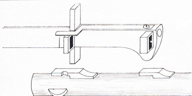
TWIN LUG METHOD OF BAYONET FIXING
